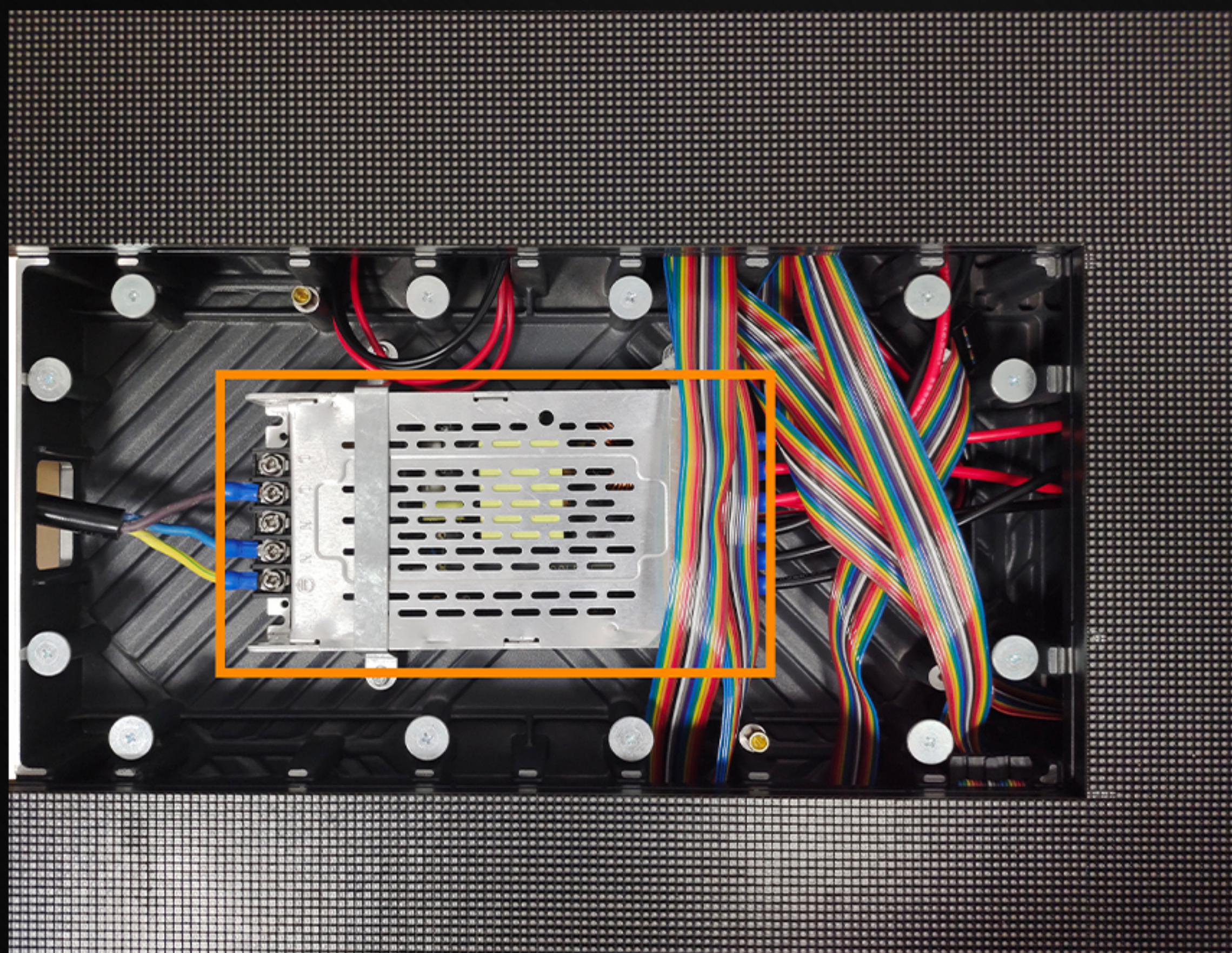
Soft Connection
